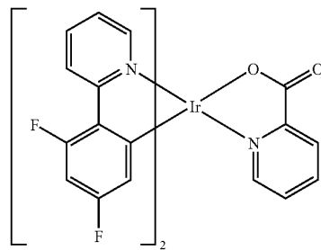
F 2 Irpic
